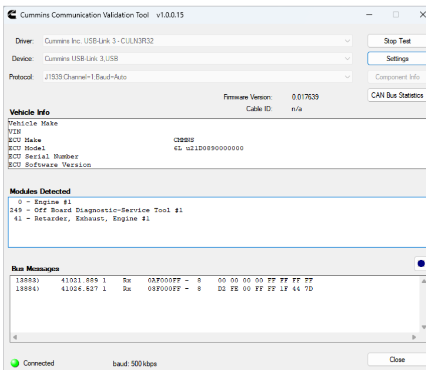
Figure 3.16 Communication Validation Tool: Status Connected
